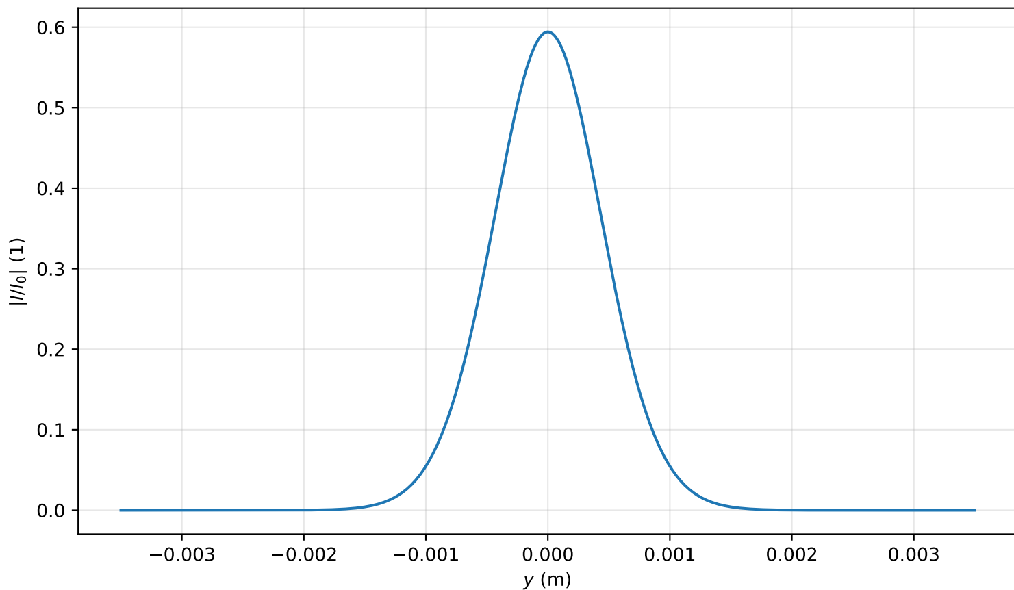
Intensity profile I(x=0, y, z=1.990)/I_0 , P_{in}=0.2P_{cr} , artificial time
